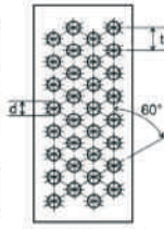
Round hole perforation in offset lines
