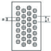
Square hole perforation in offset lines
