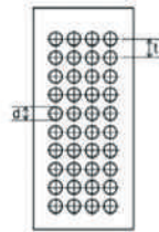
Round hole perforation in straight lines
