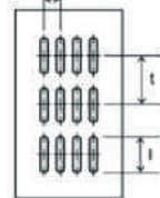
Long hole perforation in straight lines
