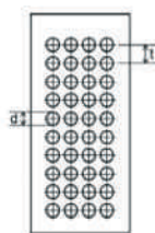
Rundlochung in geraden Reihen
